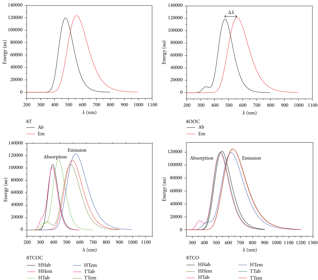
FIGURE 7: Calculated electronic absorption and emission of octamers units of 8T, 8TOC (HH, HT, and TT), 8TOOC, and 8TCOC (HH, HT, and TT) obtained by CAM-B3LYP/6-31G(d,p).
